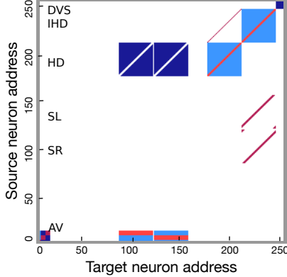
Fig. 4: The synaptic connectivity matrix that implements the architecture on the ROLLS chip. Colors encode synaptic weights of the recurrent connections on the chip (red for positive and blue for negative weights). Labels indicate the neural populations (see Fig. 3)
