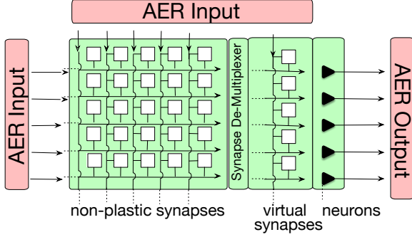
Fig. 1: Block-diagram of the chip architecture.
