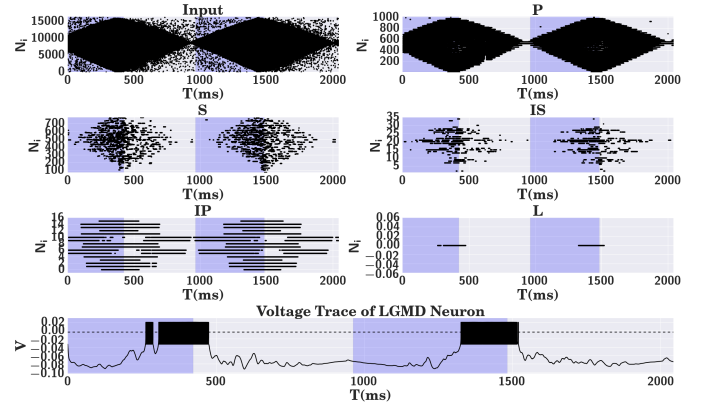
Fig. 3: Raster plots of the LGMD model layers. Last row: activation of the LGMD neuron.
